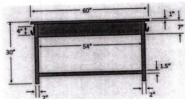
(1) Front view of the Desk
