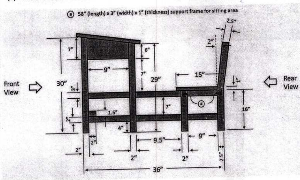
(3) Side view of the 3-seater joint desk bench
