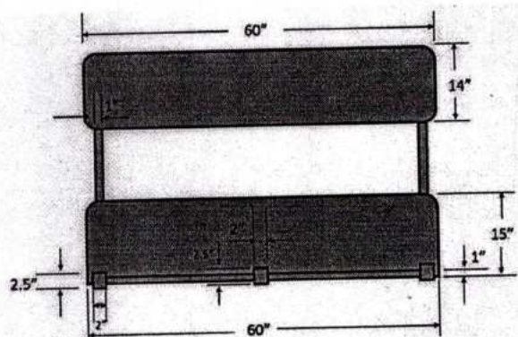
(4) Top view of the 3-seater joint desk bench
