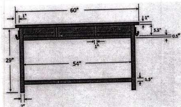
(2) Rear view of the Desk
