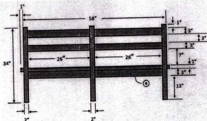
(5) Rear view of the bench
